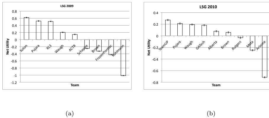
Fig. 1. The performance of the teams during the 2009 (a) and the 2010 (b) competitions. The net utility is the average utility per round minus 8, so that the average performance is zero.
