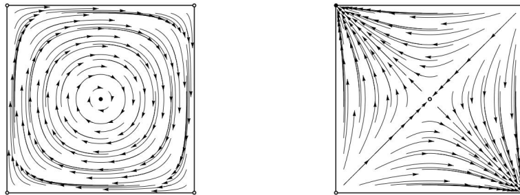
Fig. 1: Replicator trajectories in the Matching Pennies game (left) and the simple coordination game with common payoff matrix equal to -I (right). The coordinates of each point are the probabilities assigned by the players to their first strategy.
